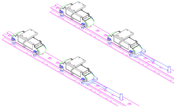
Figure 8: Modular Guide Rails (shown with RR30 rollers and pivot bearings)
