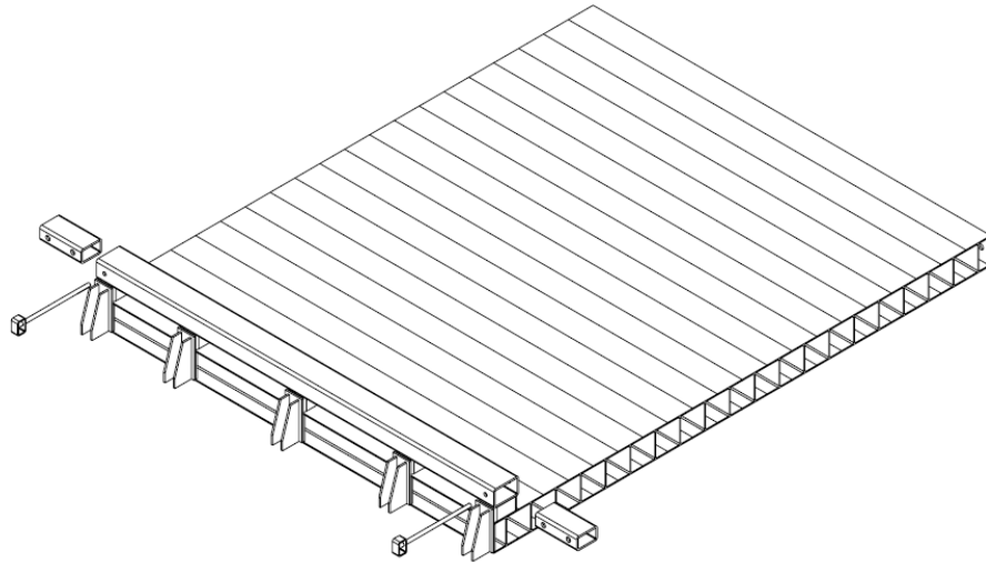
Figure 15: SSM - Structural Steel Mat (shown with optional curb system)
