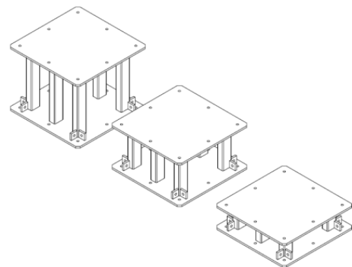
Figure 14: Support stands in varying heights
