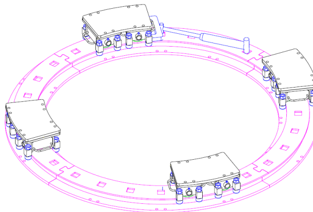
Figure 9: Modular Rotation Ring (shown with PR15 rollers and connector plates)
