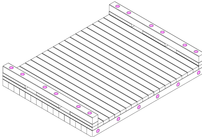
Figure 16: STM - Structural Timber Mat (shown with optional curb system)
