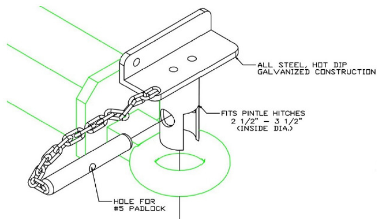
Figure 17: PHL2535 - Pintle Hitch Lock
