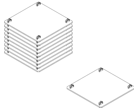
Figure 13: LDP25 load distribution plates
