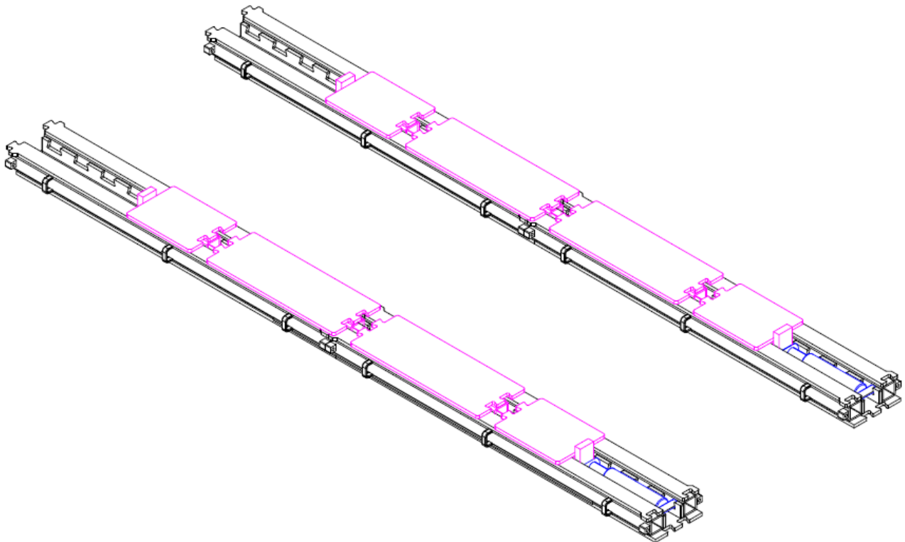
Figure 3: QC301 Quick Connect Hydraulic Skidding System (shown with optional filler shoes)
